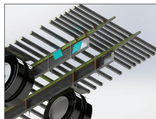
Extra Crossmembers at Rear
